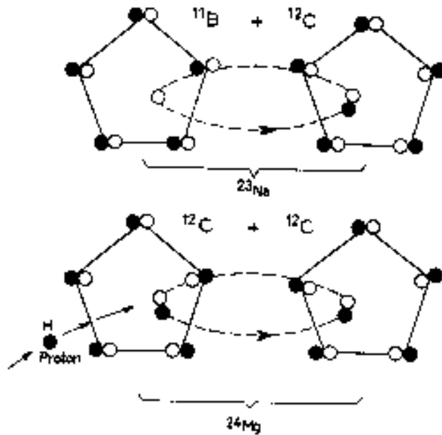
Fig.5 Passage from sodium 23 to magnesium 24: {}^{23}\text{Na} + \text{H} = {}^{24}\text{Mg} The occlusion of H would take place in the boron {}^{11}\text{B} to give carbon {}^{12}\text{C} .
